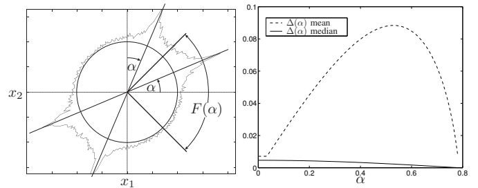
(a) circle histogram for \alpha = 0.4 (b) comparison of mean and median Fig. 1. Mean- versus median-based clustering. We consider the mixture \mathbf{x} of two independent gamma-distributed sources ( \gamma = 0.5 , 10^5 samples) using a mixing matrix \mathbf{A} with columns inclined by \alpha and (\pi/2 - \alpha) respectively. (a) shows the mixture density for \alpha = 0.4 after projection onto the circle. For \alpha \in [0, \pi/4) , (b) compares the error when estimating \mathbf{A} by the mean and the median of the projected density in the receptive field F(\alpha) = (-\pi/4, \pi/4) of the known column \mathbf{a}_1 of \mathbf{A} . The former is the k -means convergence criterion.
