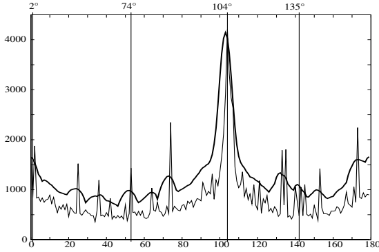
Fig. 2. Approximated probability density function of a mixture of four speech signals using the mixing angles \alpha_i = 2^\circ, 74^\circ, 104^\circ, 135^\circ . Plotted is the approximated density using a histogram with 180 bins; the thick line indicates the density after smoothing with a 5 degree radius polynomial kernel.
